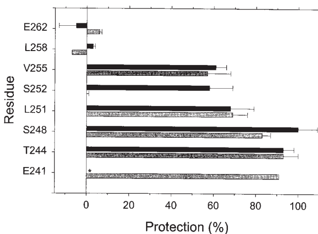
FIGURE 8. The protection by QX-314 and QX-222 of Cys-substituted residues in M2 against reaction with MTSEA. For each mutant, the rate constant of the reaction in the presence of channel blocker and ACh ( k_{\text{blocked}} ) and the rate constant of the reaction in the presence of ACh alone ( k_{\text{open}} ) were determined as described in METHODS. The extent of protection is taken as 1 - (k_{\text{blocked}}/k_{\text{open}}) . The means of two to four determinations and average errors or SEM are plotted. The lighter bars represent the protection by QX-314, and the darker bars represent the protection by QX-222. *ND.
